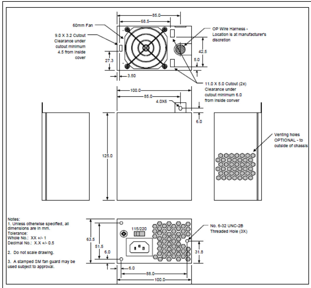
Figure 14-9: SFX12V 60 mm Mechanical Outline
