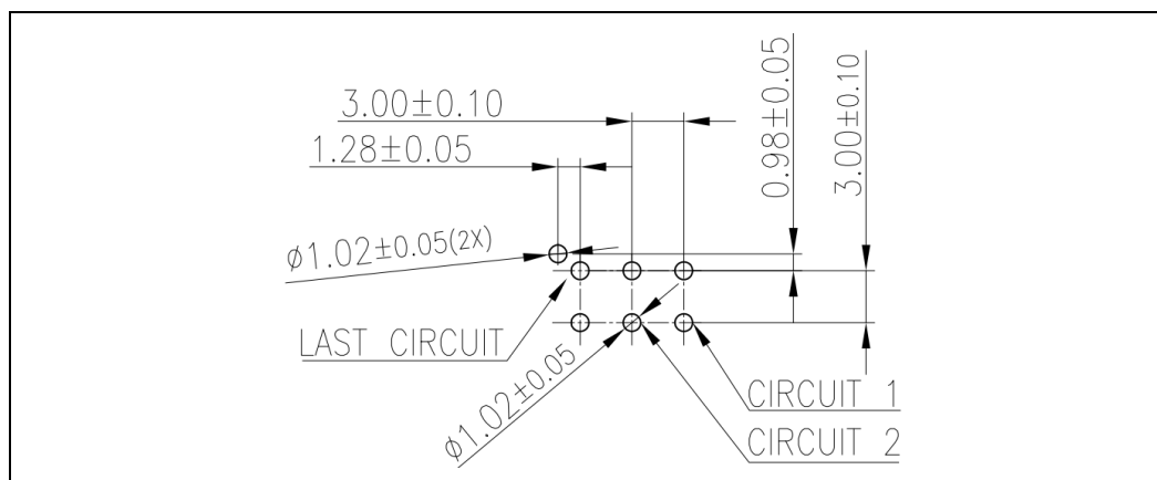
Figure 5-10: 3 mm SATA Power 6 Pin MB Header – Recommended PCB Layout (Top Layer View)
