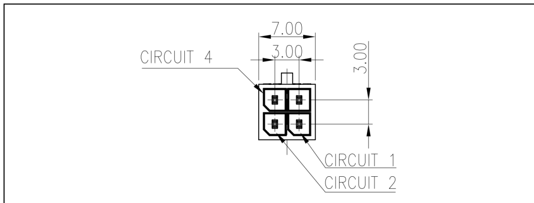
Figure 5-8: 3 mm SATA Power 4 Pin MB Header – Recommended PCB Layout (Top Layer View)
