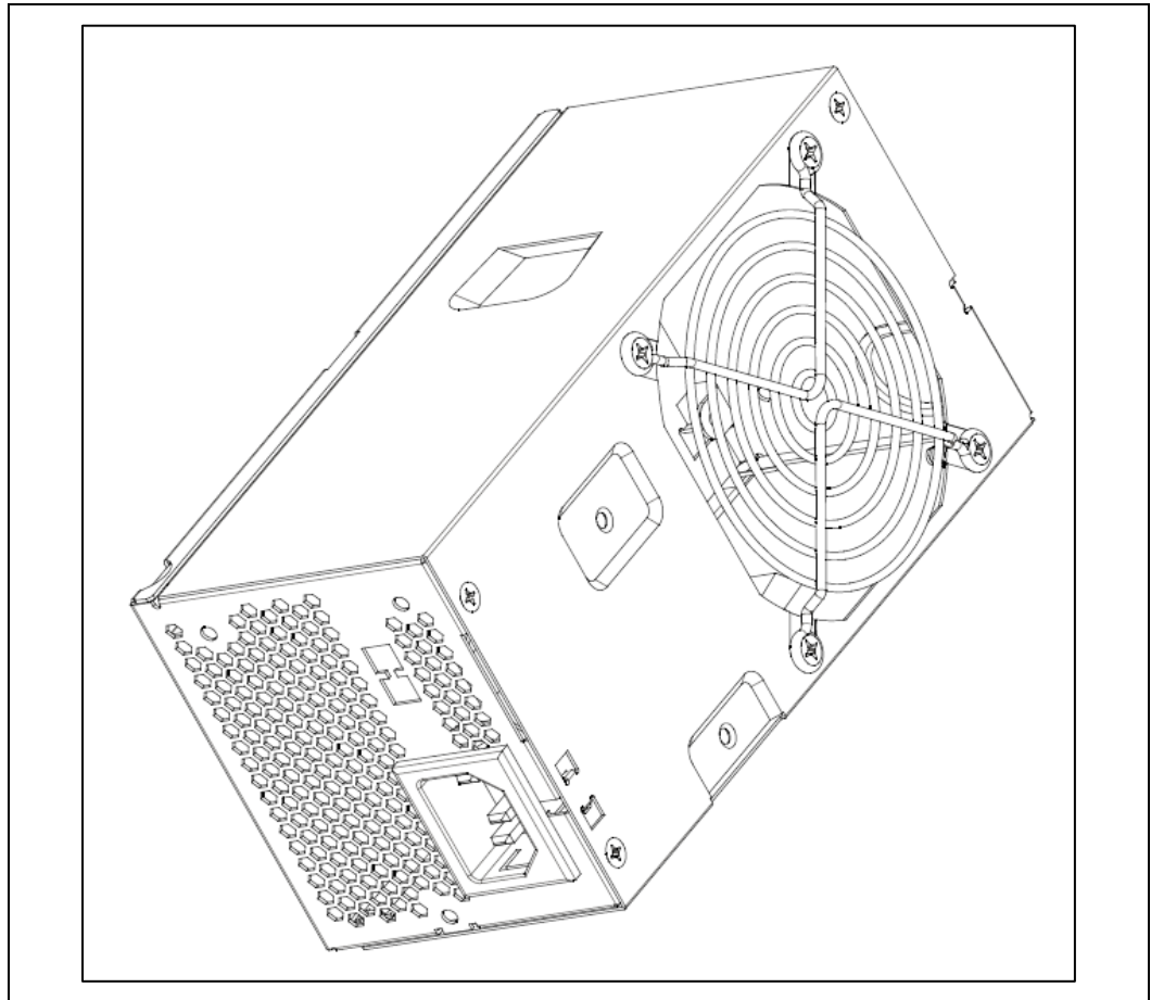
Figure 15-1: TFX12V Mechanical Outline
