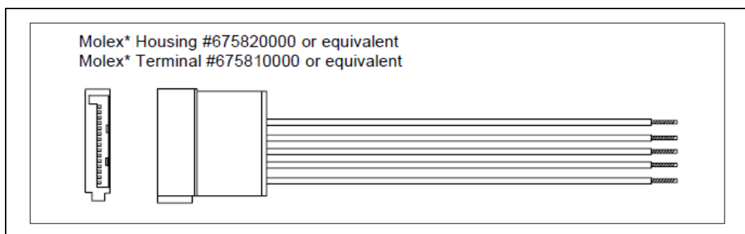
Figure 5-15: Serial ATA Power Connector
