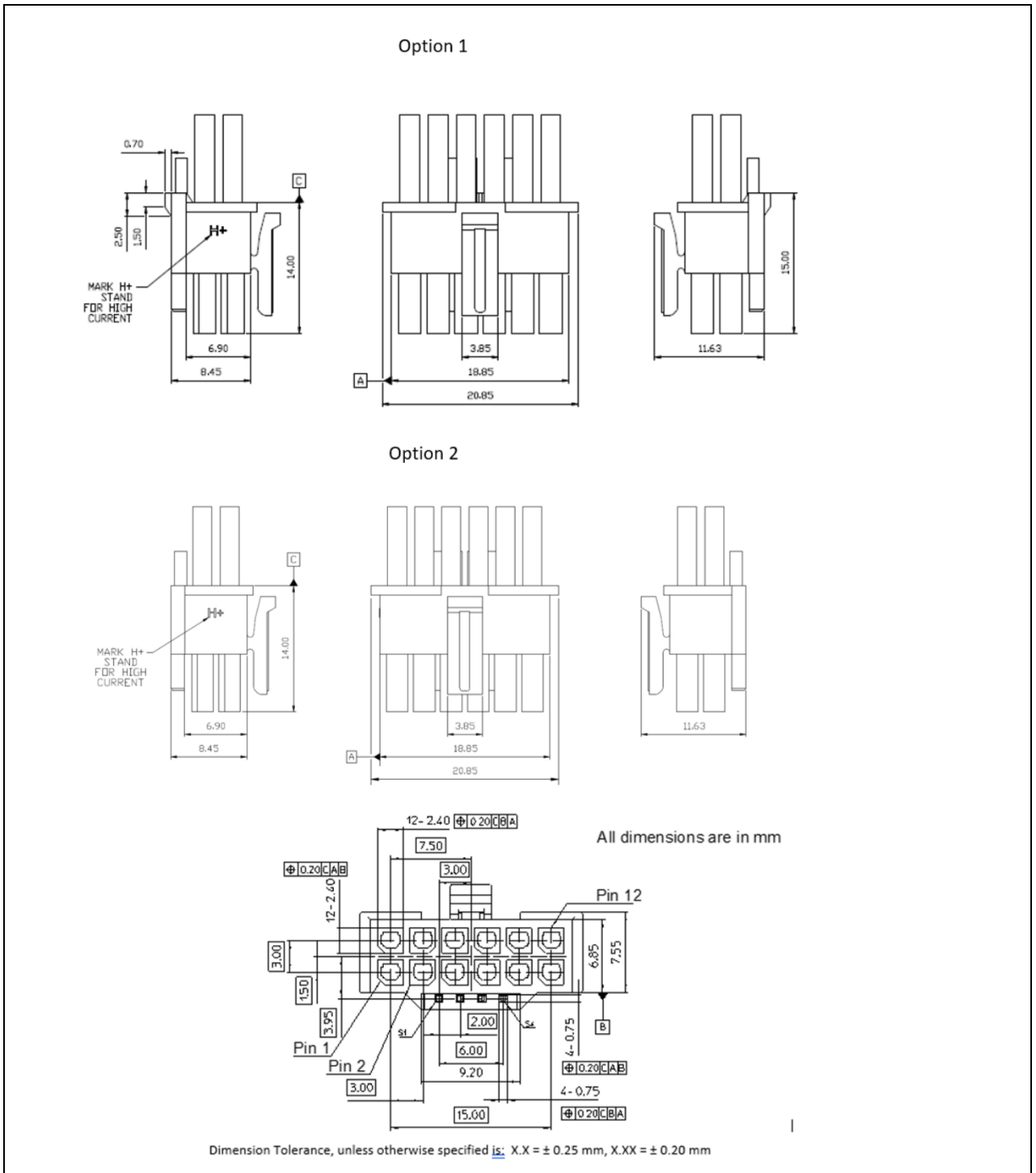
Figure 5-5: 12VHPWR Cable Assembly
