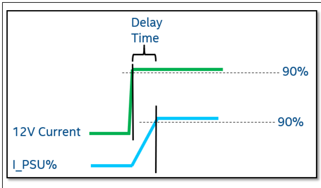
Figure 4-6: I_PSU% Delay Time Diagram
