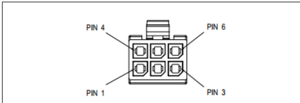
Figure 5-14: 3 mm SATA Power 6 Pin Cable Connector – Key and Pin Locations (Bottom View)
