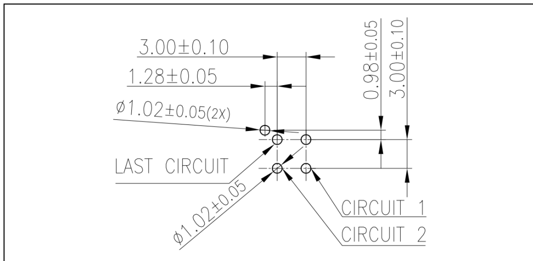
Figure 5-8: 3 mm SATA Power 4 Pin MB Header – Recommended PCB Layout (Top Layer View)
