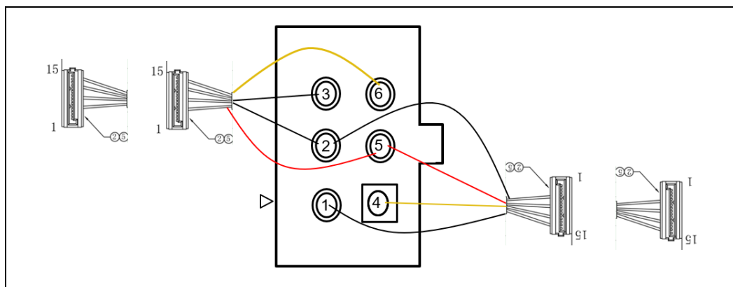
Figure 5-13: 3 mm SATA Power 6 Pin Cable Connector – Traditional Cable Diagram
