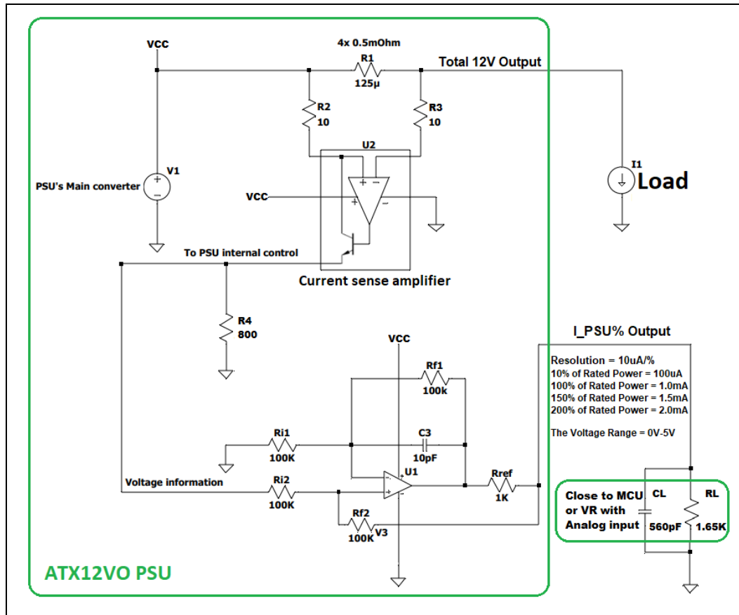
Figure 4-7: Recommended Circuit Diagram for I_PSU% signal inside PSU
