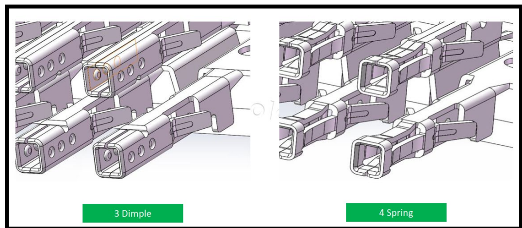
Figure 5-6: 12VHPWR Cable Plug Connection Recommendation
