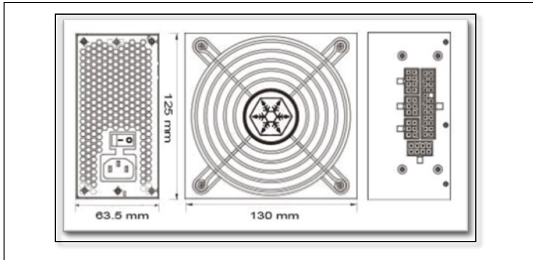
Figure 14-8: SFX12V Chassis Cutout
