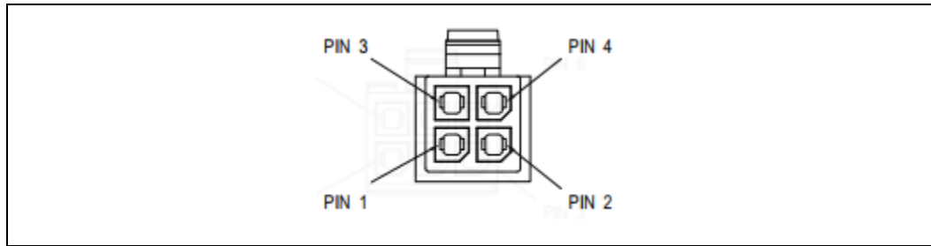
Figure 5-9: 3 mm SATA Power 4 Pin Cable Connector – Key and Pin Locations
