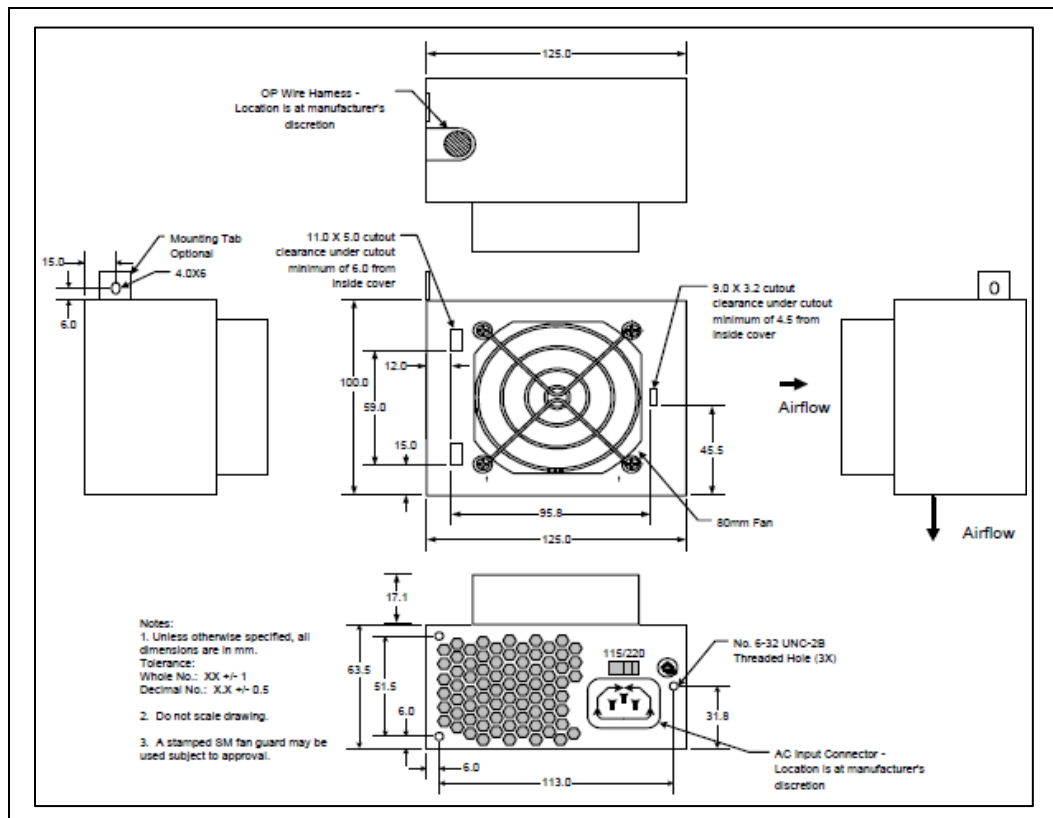
Figure 14-6: SFX12V Reduced Depth Top Mount Fan Profile Mechanical Outline
