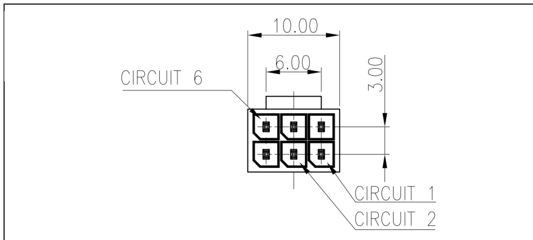
Figure 5-11: 3 mm SATA Power 6 Pin MB Header – Keying and Pin Locations
