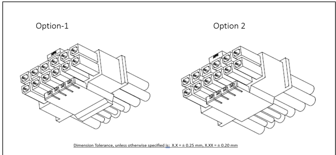
Figure 5-4: 12VHPWR Cable Plug Connector
