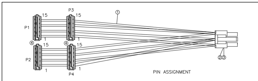
Figure 5-13: 3 mm SATA Power 6 Pin Cable Connector – Traditional Cable Diagram
